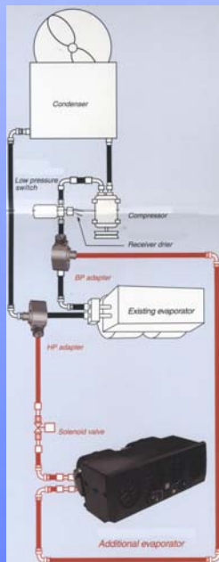
Complete kit for additional AC system to connect to OE dash A/C system
